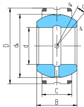
GEC..X
