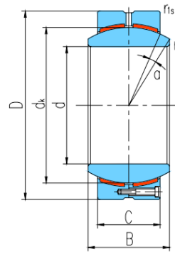
GEC...HC
