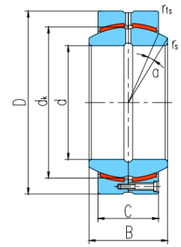
GEC...HCS
