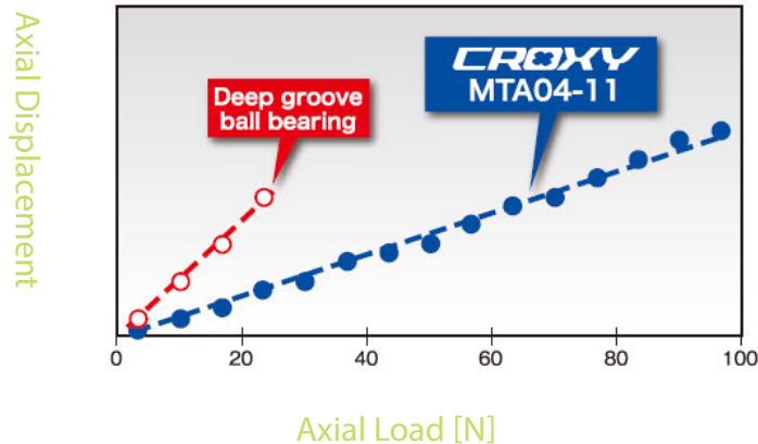
Axial Displacement Comparison (IdØ4mm)
